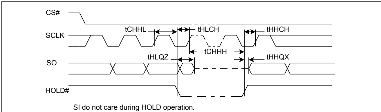
Figure 46. Hold Timing
